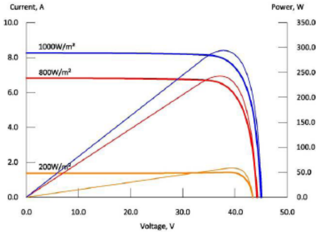
Current-Voltage & Power-Voltage characteristics various irradiance levels
